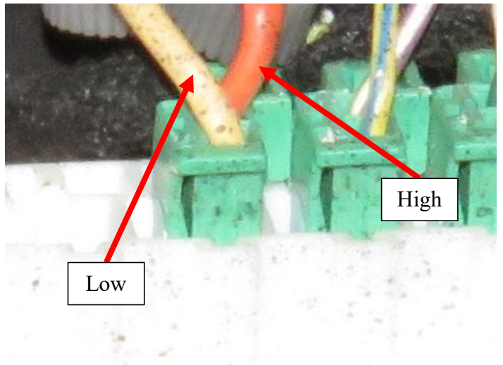
Use wire taps on wires from this plug
