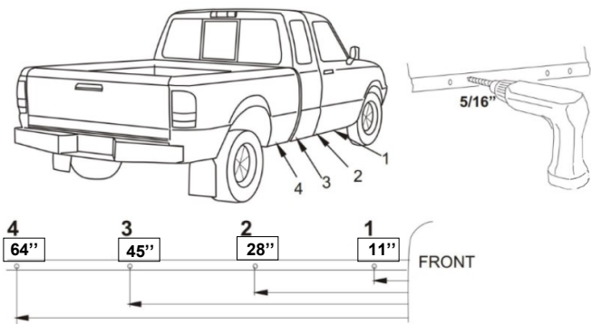
(Fig 1) Passenger Side Mounting Locations
