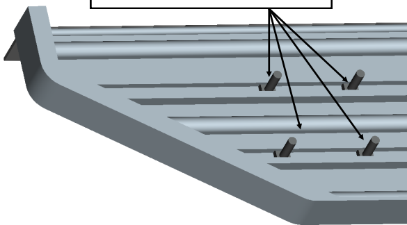
(Fig 4) Slip (3) M6X1-20mm Square Head Bolts Into Each Bottom Channel
