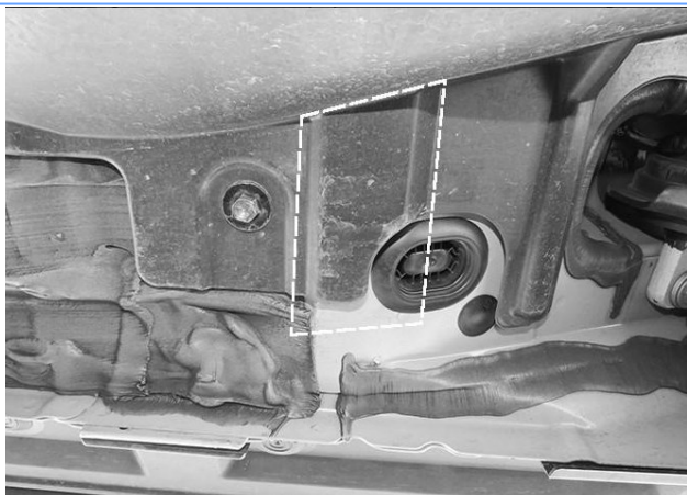
(Fig 7) Passenger Rear mounting location cut along dotted lines
