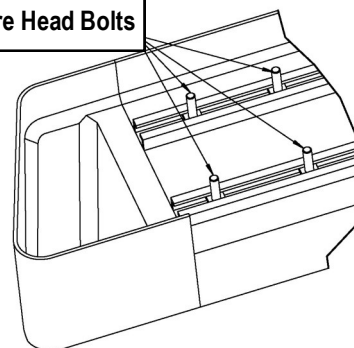
(Fig 18) Slip M6X1-20mm Square Head Bolts Into The Bottom Channels
