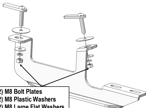
(Fig 16) M8 Bolt Plates Installed into Passenger Rear Mounting Holes
