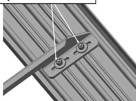
(Fig 19) Running Board Installed Onto Mounting Bracket
