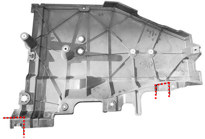
(Fig 22) Driver Rear Underside Cover Cut lines
