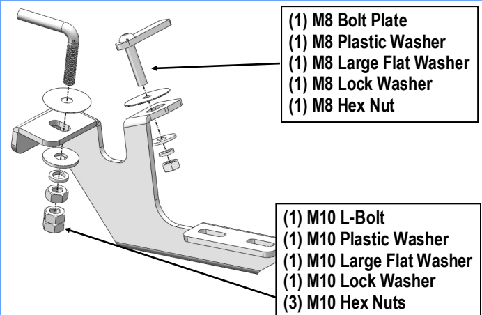
(Fig 14) Passenger Center Mounting Brackets Installation
