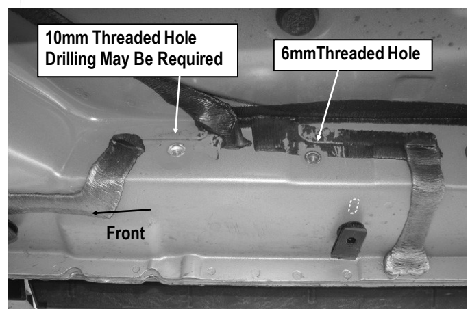
(Fig 6) Passenger Side Front Mounting Location
