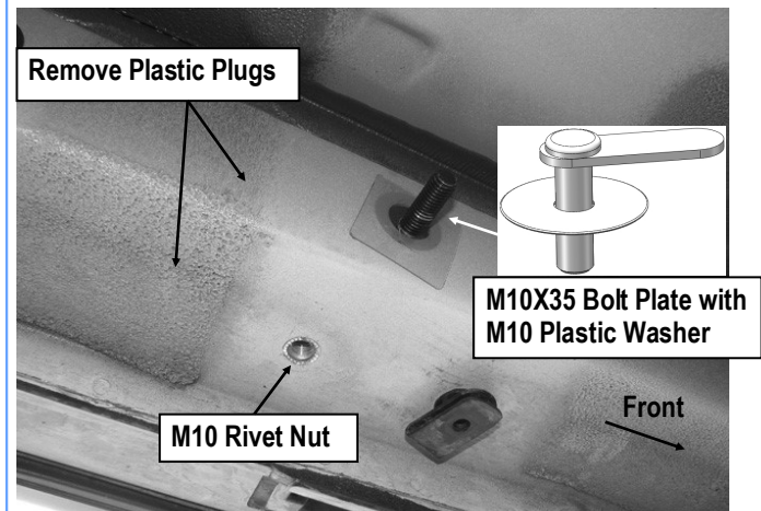
(Fig 9) Driver Side Center Mounting Location
