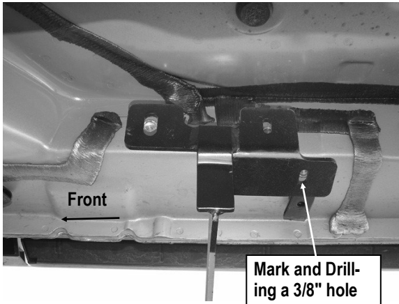
(Fig 7) Passenger Side Front Mounting Location
