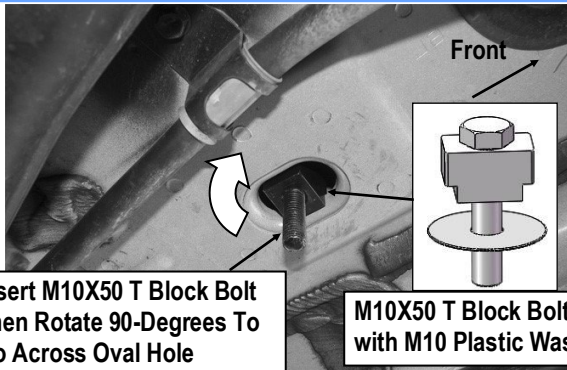
(Fig 15) Driver Side Rear Mounting Location
