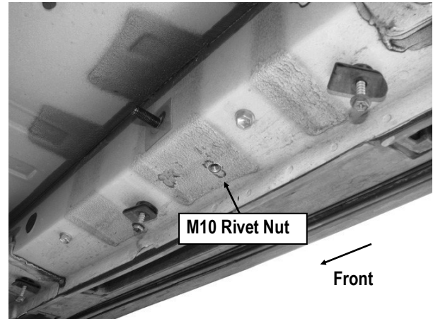
(Fig 13) Passenger Side Center Mounting Location
