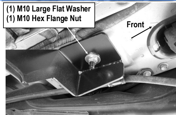
(Fig 16) Driver Side Rear Mounting Location
