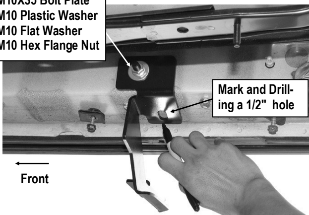
(Fig 11) Passenger Side Center Mounting Location
