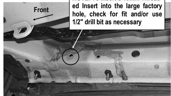
(Fig 5) Passenger Side Front Mounting Location
