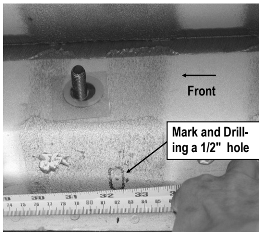
(Fig 12) Passenger Side Center Mounting Location
