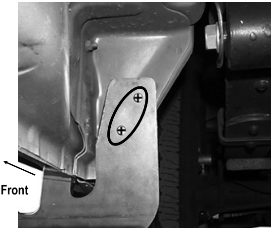
(Fig 12) Mark The Location Of the (2) Mounting Holes
