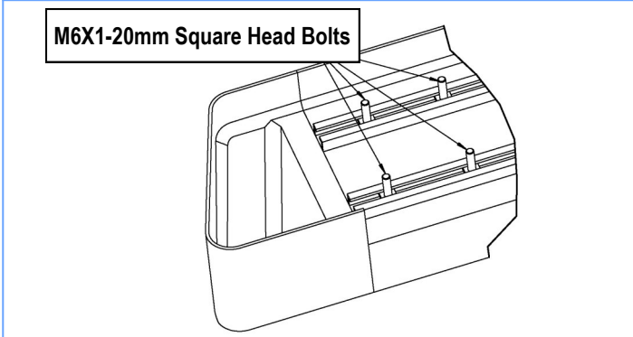
(Fig 10) Slip M6X1-20mm Square Head Bolts Into The Bottom Channels
