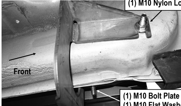
(Fig 17) Driver Front Mounting Bracket Installation
