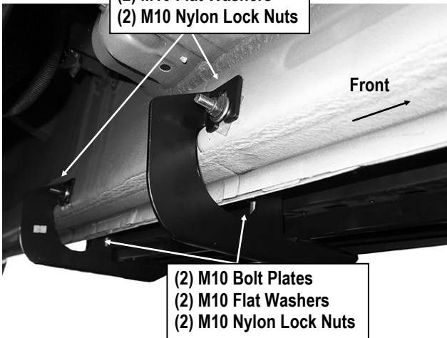
(Fig 18) Driver Center & Rear Mounting Bracket Installation
