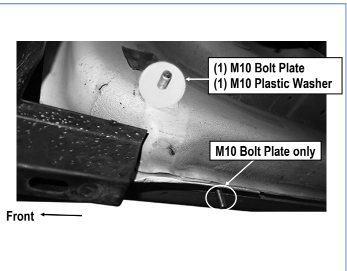
(Fig 2) Passenger Front Mounting Bracket Location
