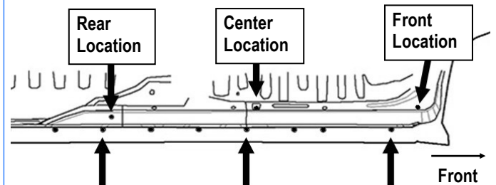
(Fig 15) Driver Side (3) Mounting Locations
