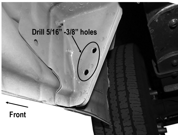
(Fig 13) Drill Holes on Passenger Side Rear Mounting Location
