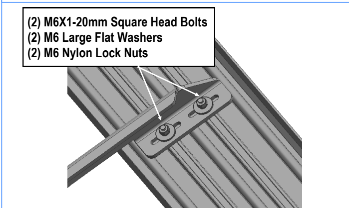
(Fig 11) Running Board Installed Onto Mounting Bracket (Example)
