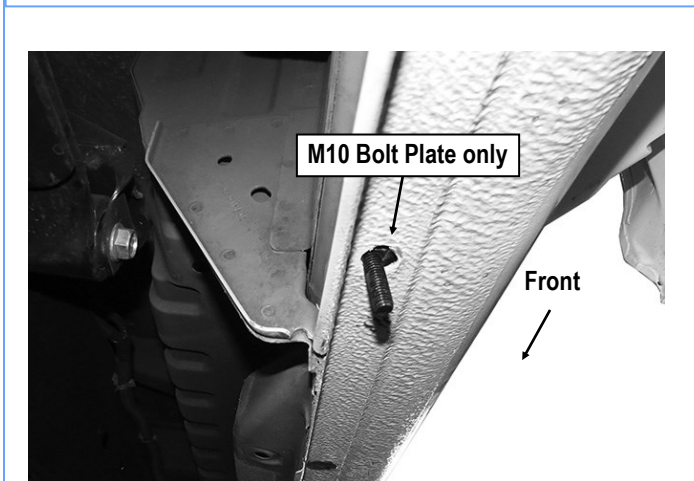
(Fig 9) Passenger Rear Mounting Bracket Location
