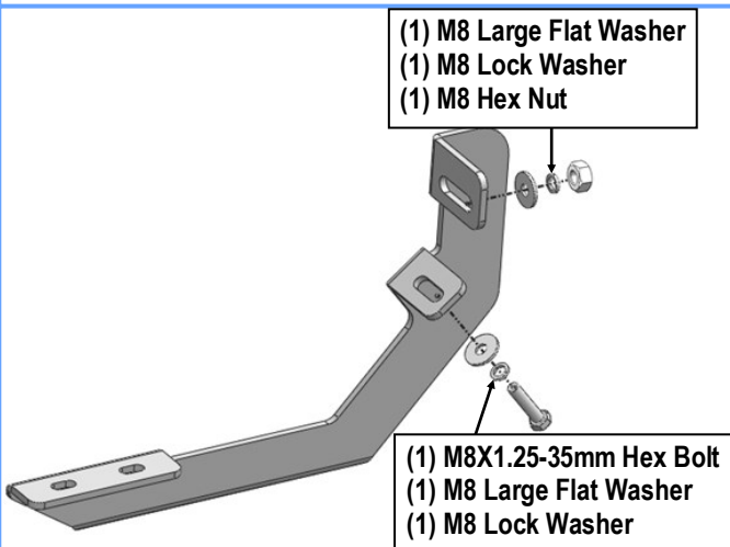
(Fig 2) Driver Side Front Mounting Bracket Installation
