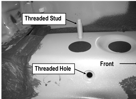
(Fig 1) Driver Side Front Mounting Bracket Location
