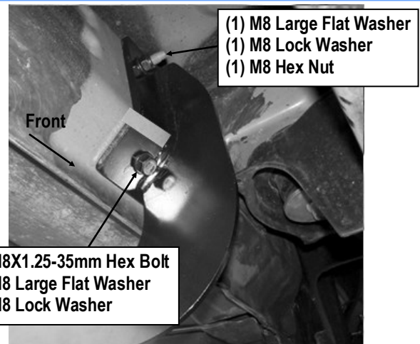
(Fig 3) Driver Side Front Mounting Bracket Installation
