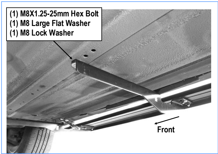
(Fig 13) Passenger Center Mounting Bracket Installation
