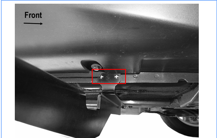
(Fig 14) Passenger Front Bracket Location Marked Before Drilling
