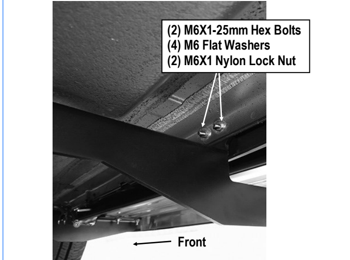
(Fig 17) Passenger Center Mounting Bracket Installation
