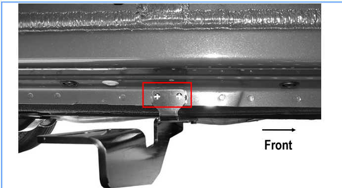
(Fig 15) Passenger Center Bracket Location Marked Before Drilling (Rocker Panel Cover Removed)
