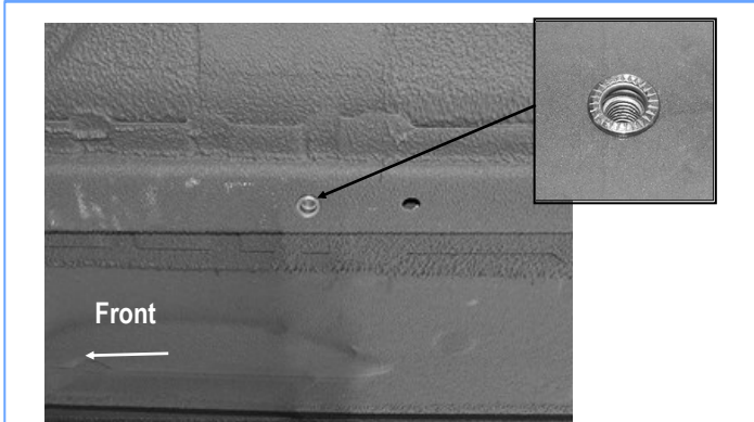
(Fig 12) Insert The M8 Rivet Nut
