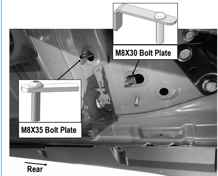
(Fig 5) Insert M8X35 Bolt Plate & M8X30 Bolt Plate
