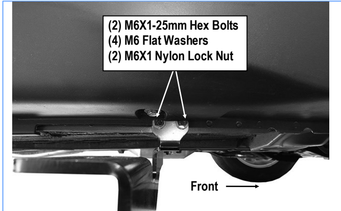
(Fig 16) Passenger Front Mounting Bracket Installation
