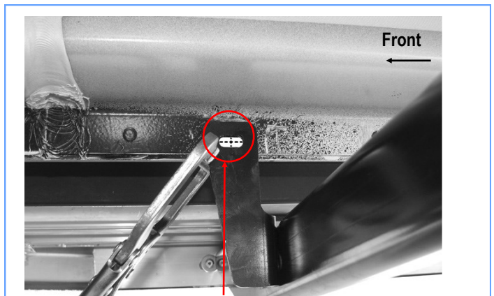
(Fig 14) Marking And Drilling Holes (Passenger Side Front Mounting Bracket )
