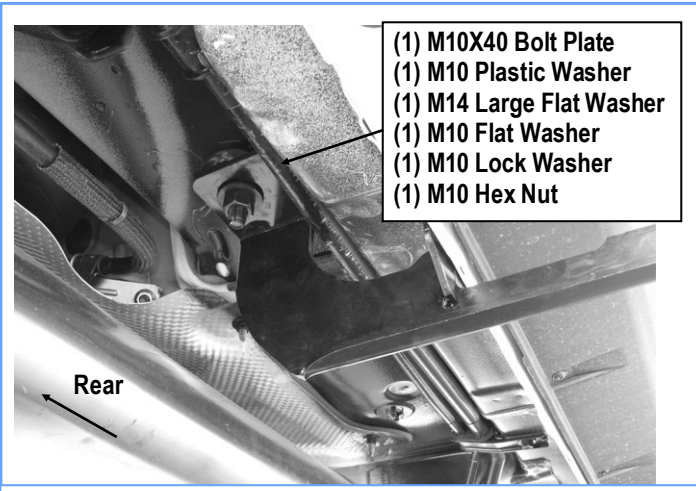
(Fig 11) Passenger Side Rear Mounting Bracket Installation
