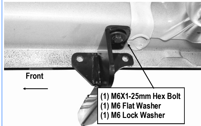
(Fig 7) Passenger Side Center Mounting Bracket Installation
