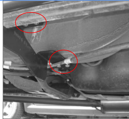
(Fig 3) Driver Rear Mounting Bracket Installed
