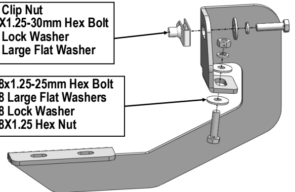
(Fig 4) Driver Rear Mounting Bracket Installation
