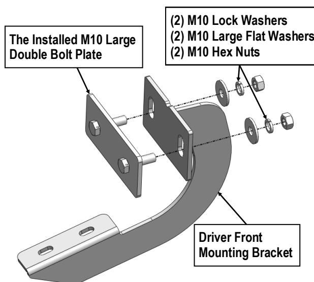
(Fig 4) Driver Front Mounting Bracket Installation
