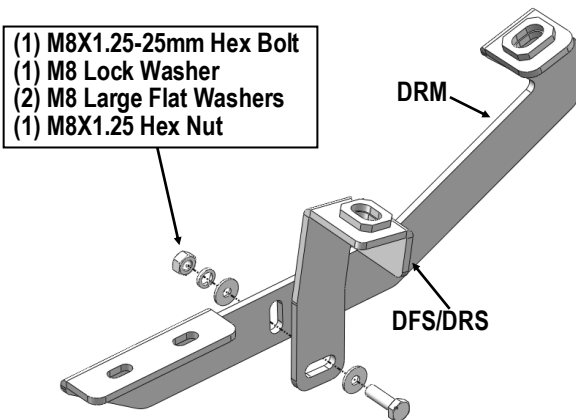
(Fig 12) Driver Side Rear Brackets Assembly
