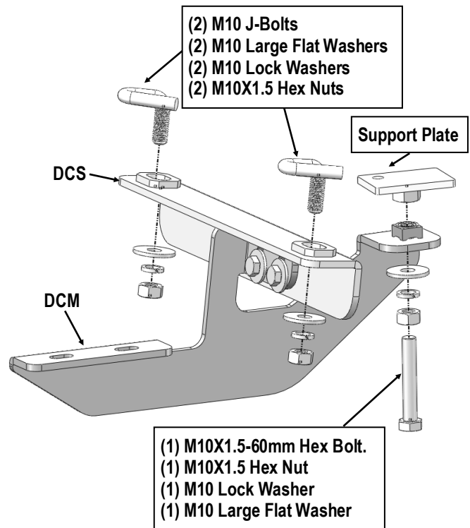
(Fig 9) Driver Side Center Brackets Installation
