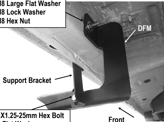
(Fig 11) Passenger Side Front Bracket Installation
