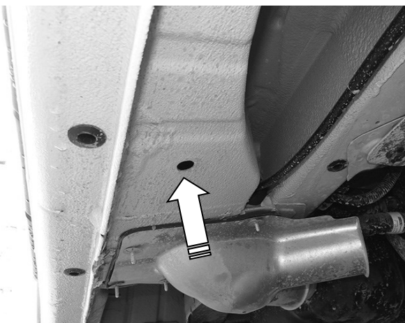
(Fig 4) Driver Side Rear Mounting Bracket Location
