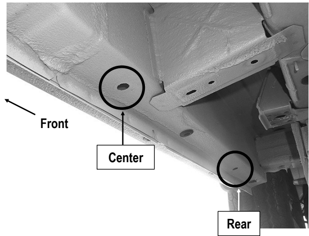
(Fig 12) Passenger Side Center & Rear Mounting Locations
