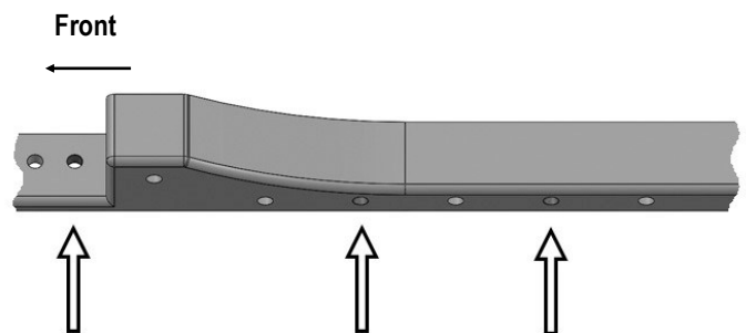
(Fig 10A) Passenger Side Mounting Bracket Locations
