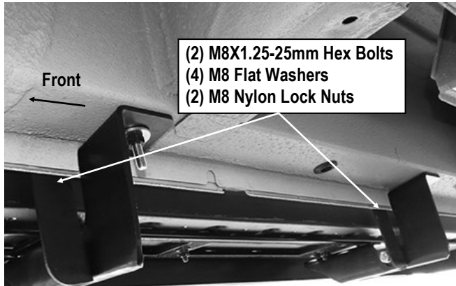
(Fig 14) Attach Passenger Center & Rear Support Bracket To Pinch Weld
