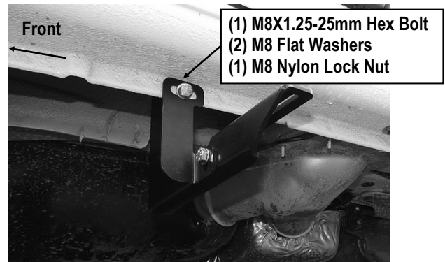
(Fig 9) Attach Driver Side Support Bracket To Pinch Weld
