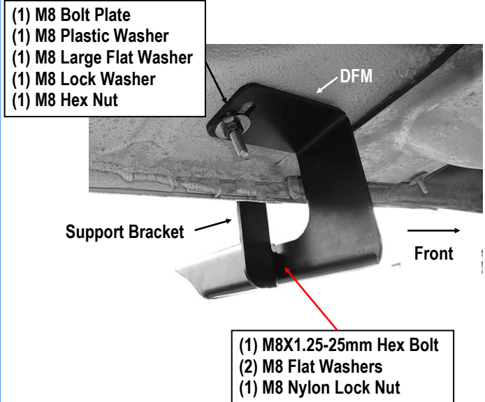
(Fig 5) Driver Rear Mounting Bracket Installation
