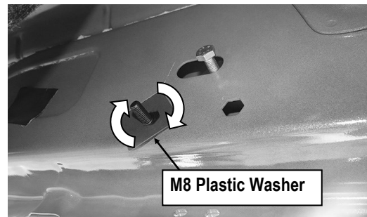
(Fig 5) Thread Plastic Washer Onto the Welded Bolt on M8 Bolt/Nut Plate To Hold Bolt/Nut Plate In Position. IMPORTANT: Do Not Remove The Hex Bolt Until The M8 Plastic Washer Has Been Threaded Onto the Welded Bolt.
