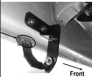
(Fig 10B) Attach Driver Front Support Bracket To the Back Of Pinch Weld (Models With Factory Holes In Pinch Weld Only)
