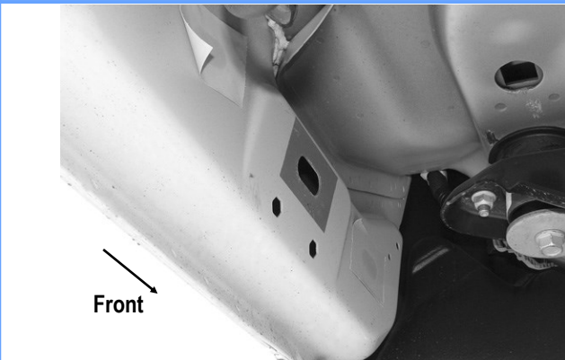
(Fig 1) Driver Side Front Mounting Location (No Factory Holes In Pinch Weld on Some Models)
