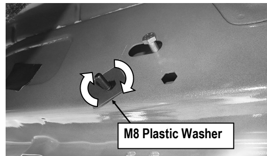
(Fig 5) Thread Plastic Washer Onto the Welded Bolt on M8 Bolt/Nut Plate To Hold Bolt/Nut Plate In Position.
