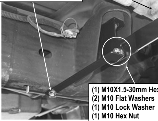
(Fig 8) Passenger Front Support Bracket Installed (Up to 2011 2500/3500 Models )
