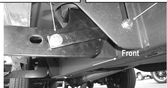
(Fig 9) Passenger Side Center Bracket Installed (1500 Models)
