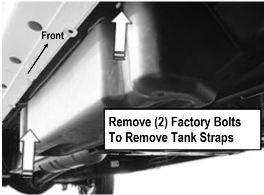
(Fig 12) 07-16 Passenger Side DEF Tank And Cover
