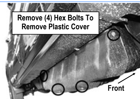
(Fig 11A) 2017-Up Passenger Side Pictured With DEF Plastic Tank Cover.
