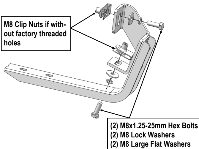
(Fig 7) Driver Front Brackets Installation
