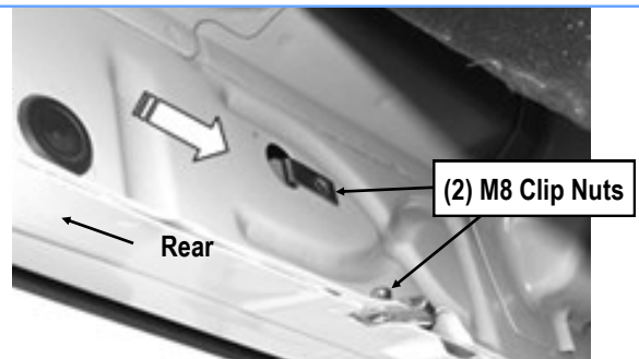
(Fig 4) Driver Side Rear Center Mounting Location
