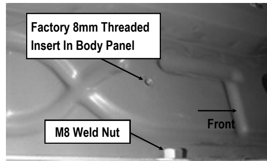
(Fig 2) Driver Side Front Mounting Location
