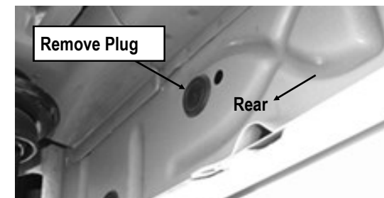
(Fig 4) Driver Side Rear Center Mounting Location
