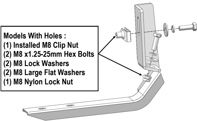
(Fig 13) Passenger Front Mounting Bracket Installation
