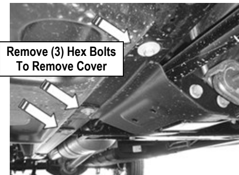
(Fig 10) 07-16 Passenger Side Front With DEF Tank Cover
