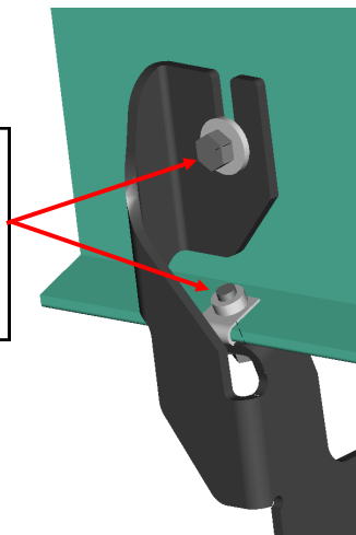
(Fig 12) Passenger Front Mounting Bracket Installed
