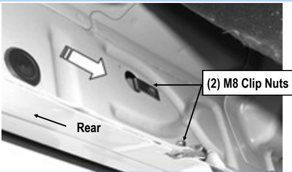
(Fig 5) Driver Side Rear Mounting Location
