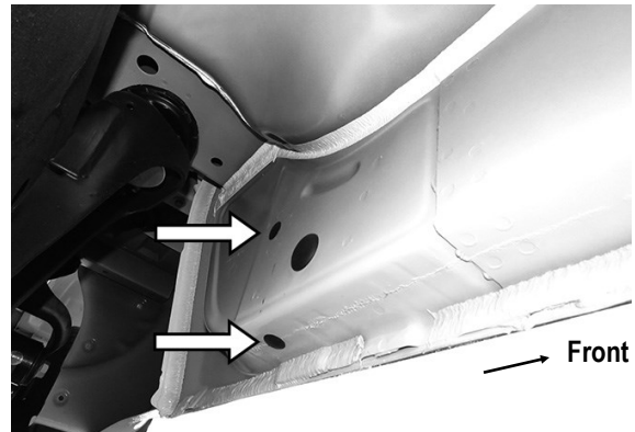
(Fig 5) Driver Rear Side Mounting Location
