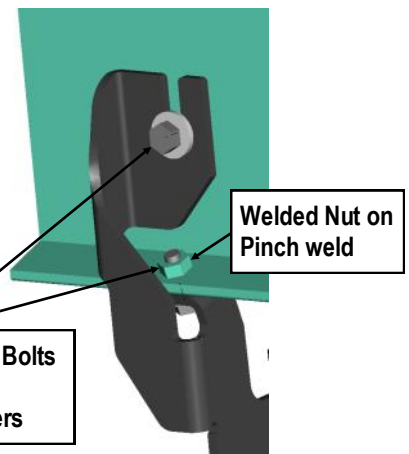
(Fig 13) Passenger Front Mounting Bracket Installed (Models with welded nut/ threaded insert)
