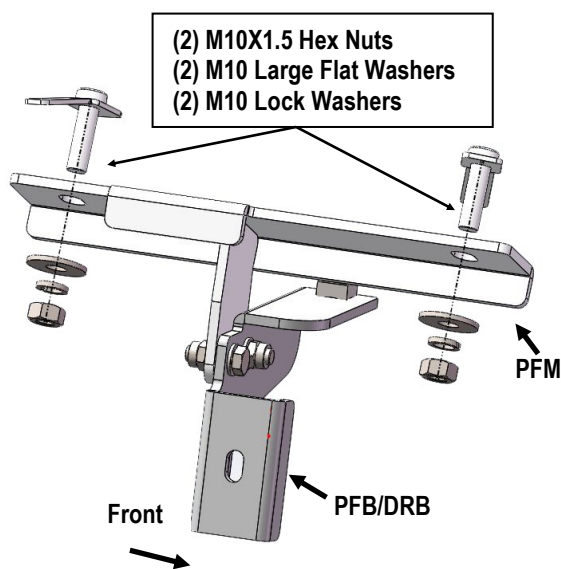
(Fig 5) Passenger Front Mounting Bracket (PFM) Installation
