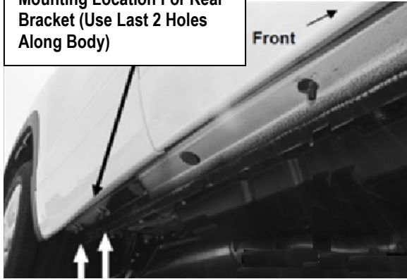
(Fig 7) Passenger Side Rear Bracket Location
