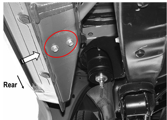
(Fig 7) Passenger Side Rear Mounting Location
