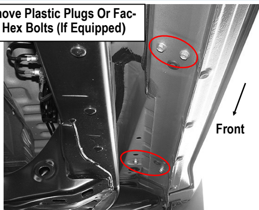
(Fig 1) Passenger Side Front & Center Mounting Location
