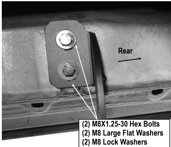
(Fig 8) Passenger Rear Mounting Bracket Installed
