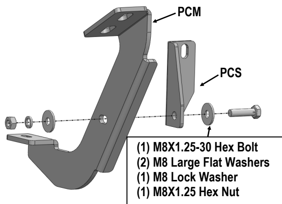
(Fig 5) Passenger Center Mounting Bracket Assembly
