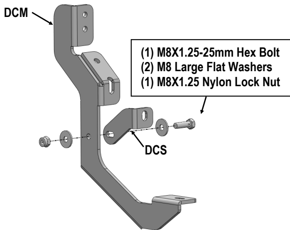
(Fig 3) Driver Center Brackets Assembly
