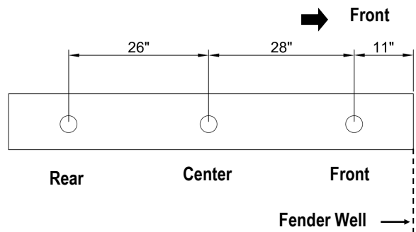
(Fig 1) Driver Side Mounting Locations (on Pinch Weld)
