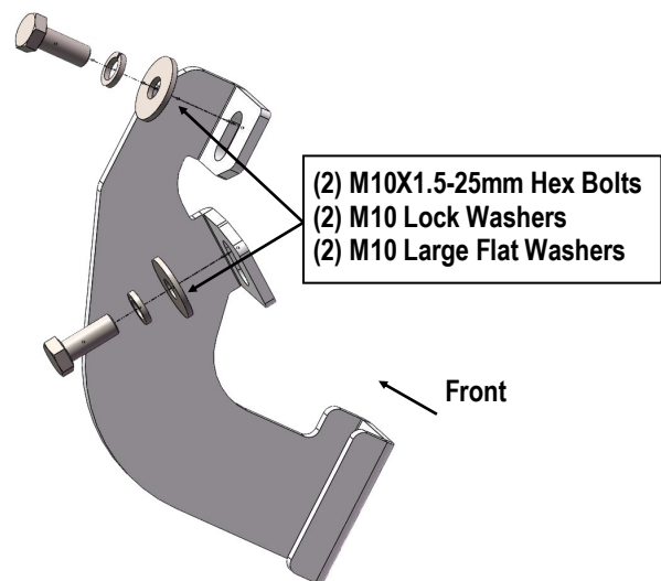
(Fig 4) Passenger Center Mounting Bracket (PCM/PRM) Installation
