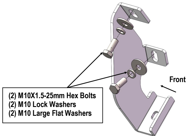
(Fig 2) Passenger Front Mounting Bracket (PFM) Installation
