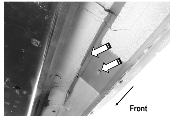
(Fig 3) Passenger Side Center Mounting Location
