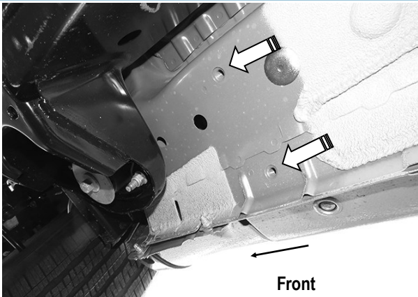
(Fig 1) Passenger Front Mounting Location
