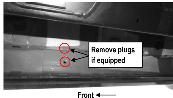
(Fig 3) Passenger Side Center Mounting Location
