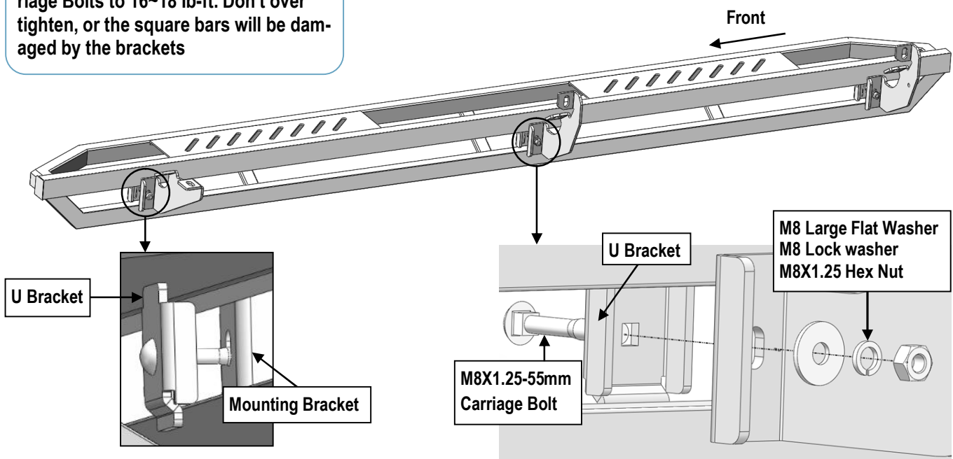
(Fig 6) Passenger Side Step Bar Installation
