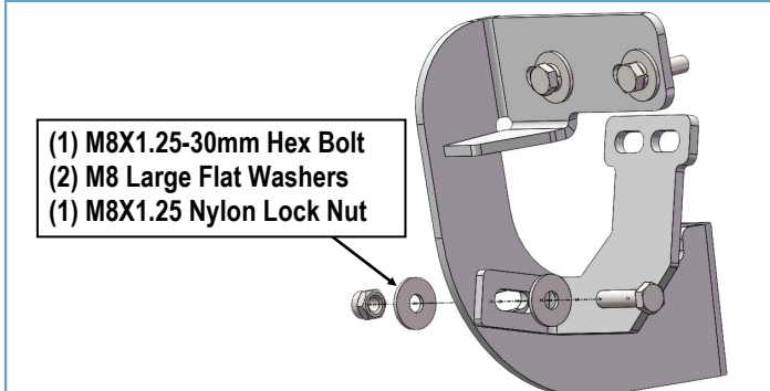
(Fig 9) Attach Driver Front Support Bracket To Front Facing Side Of the Driver Front Mounting Bracket
