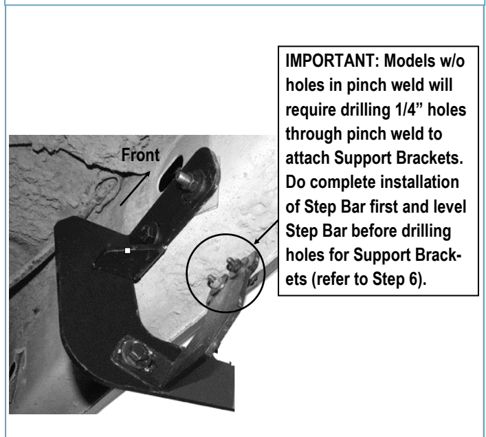
(Fig 10B) Driver Front Brackets installed
