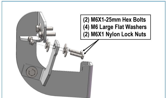
(Fig 10A) Attach Driver Front Support Bracket To the Back Of The Pinch Weld (Models With Factory Holes In Pinch Weld Only)
