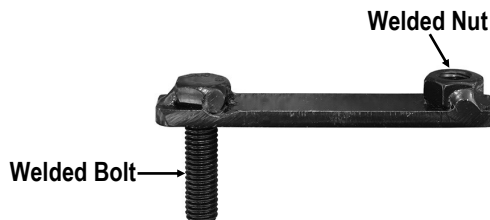
(Fig 2) M8 Bolt/Nut Plate (NOTE: M8 Bolt/Nut Plate Is Not Required On Models With Factory Threaded Inserts)
