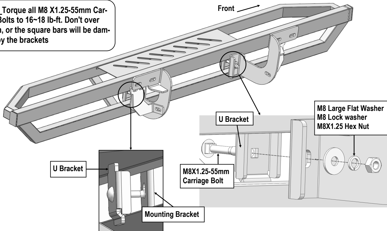
(Fig 13) Driver Side Step Bar Installation
