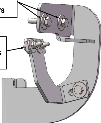
(Fig 12A) Driver Rear Brackets Installed
