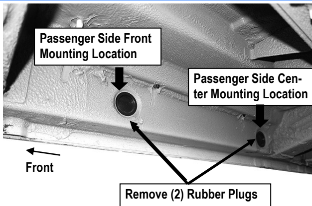
(Fig 1) Passenger Side Front & Center Mounting Locations
