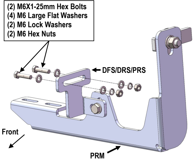
(Fig 11) Attach Support Bracket To Pinch Weld
