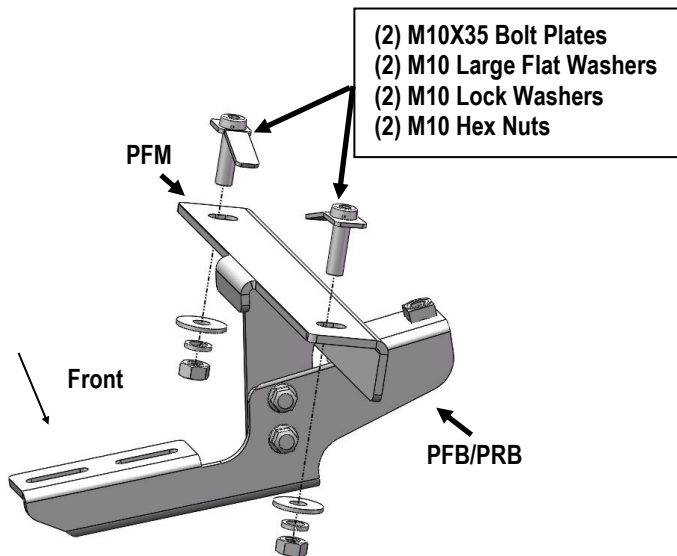
(Fig 4) Passenger Front Mounting Bracket Installation
