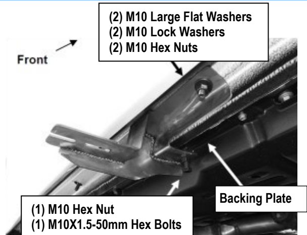
(Fig 6) Passenger Front Bar Bracket Installation
