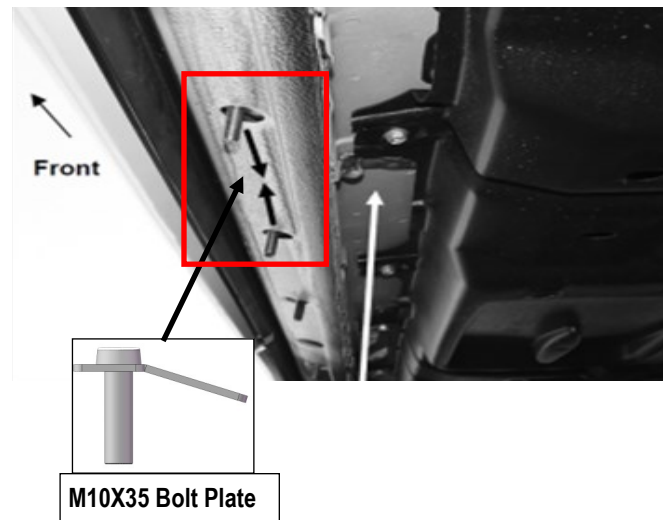
(Fig 2) Insert M10X35 Bolt Plate
