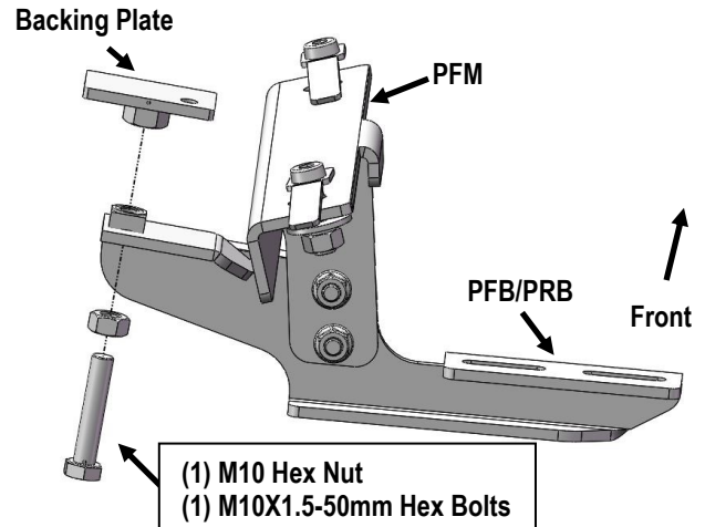
(Fig 5) Passenger Front Bar Bracket Installation
