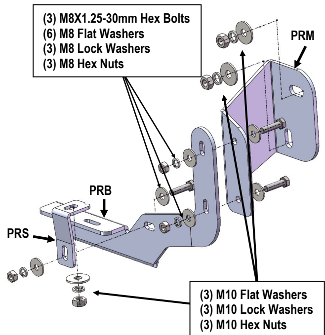
(Fig 20) Passenger Side Rear Bracket Location Pictured
