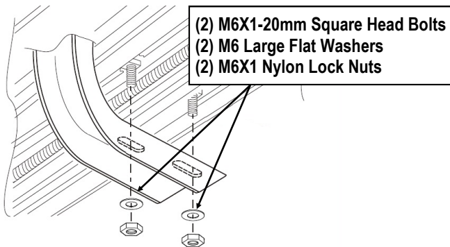
(Fig 22) Running Board Installed Onto Mounting Bracket
