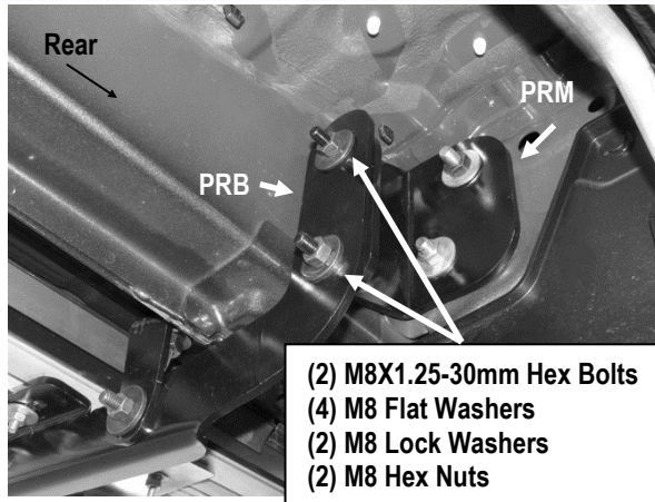
(Fig 18) Passenger Rear Mounting Bracket (PRM) And Passenger Rear Bar Bracket (PRB) Assembly
