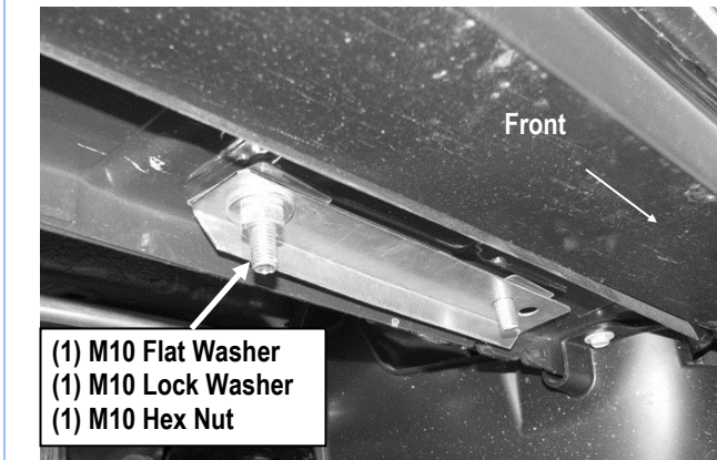
(Fig 4) Mounting Plate Installation
