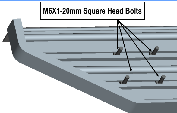
(Fig 21) Slip M6X1-20mm Square Head Bolts Into The Bottom Channels
