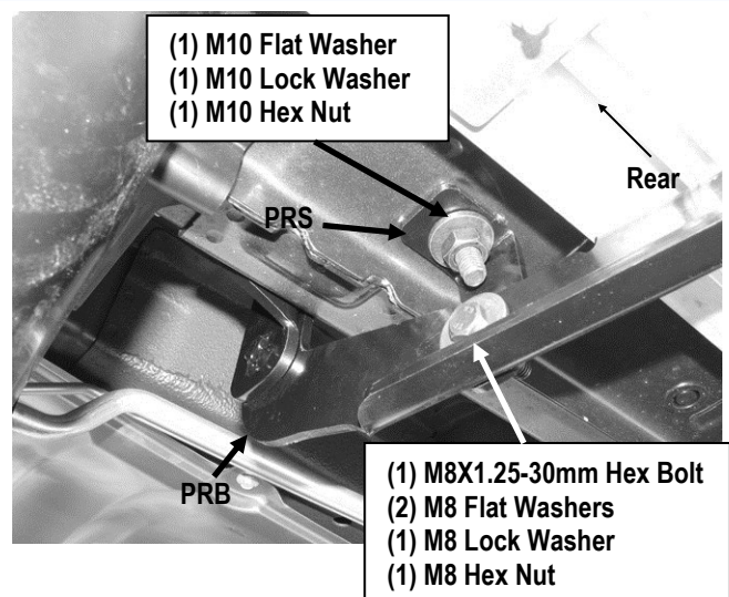
(Fig 19) Passenger Rear 7 Support Bracket (DRS/PRS) Installation
