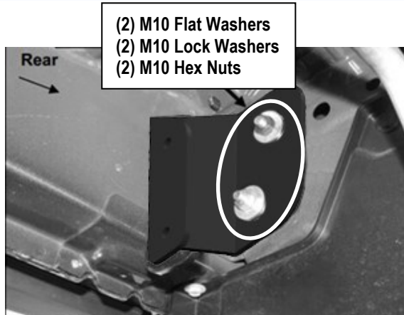
(Fig 17) Passenger Rear Mounting Bracket (PRM) Installation
