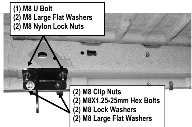
(Fig 23) Driver Rear Mounting Bracket (DRM) Installed
