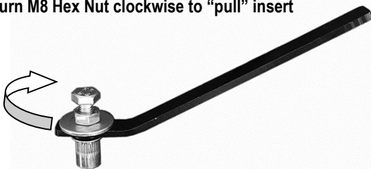
(Fig 19) M8 Insert Tool Assembly
