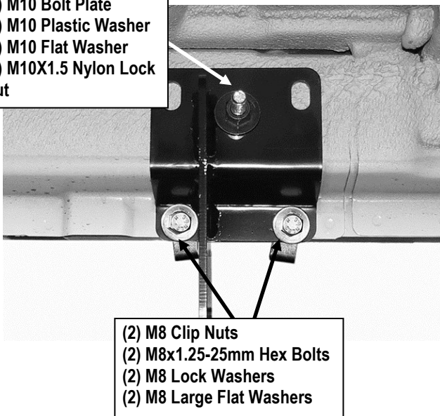
(Fig 7) Passenger Side Front Mounting Bracket Installation
