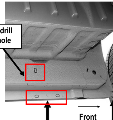
Mark and drill (2) 3/8" holes through pinch weld
