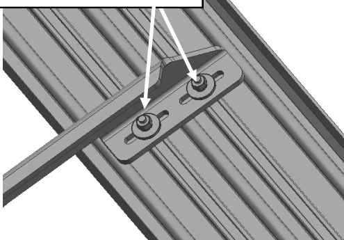
(Fig 15) Running Board Installed Onto Mounting Bracket
