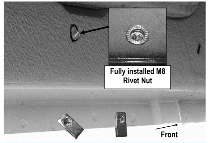
(Fig 20) Driver Side Front Mounting Location
