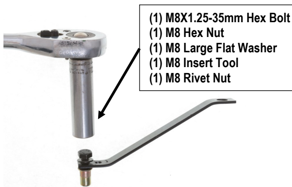
(Fig 17) M8 Insert Tool Assembly
