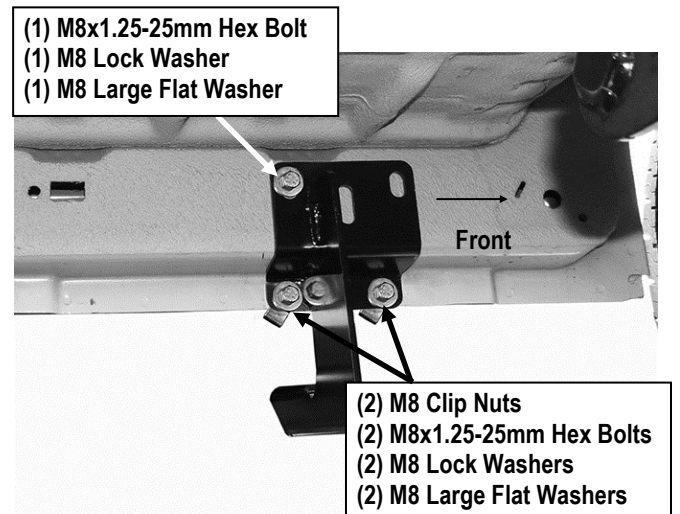
(Fig 21) Driver Front Mounting Bracket Installed
