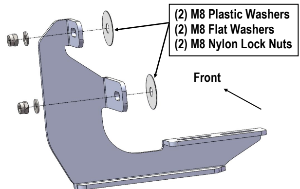
(Fig 3) Passenger Front Mounting Bracket (DFM/PFM) Installation
