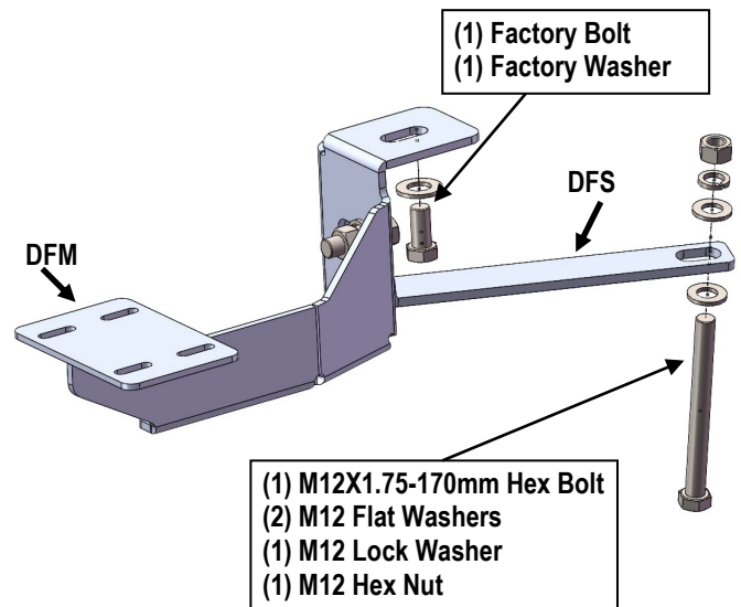
(Fig 2) Driver Front Mounting Brackets Installation
