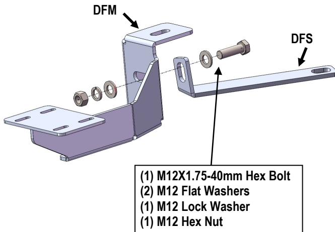
(Fig 1) Driver Side Front Mounting Bracket Assembly
