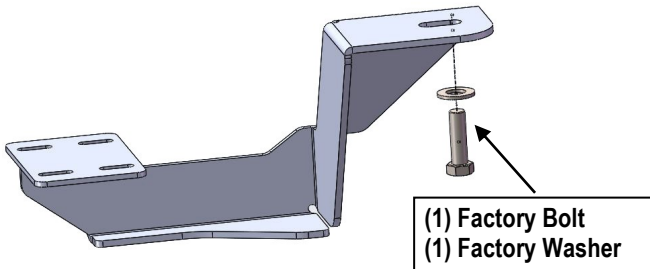
(Fig 3) Driver Rear Mounting Bracket Installation
