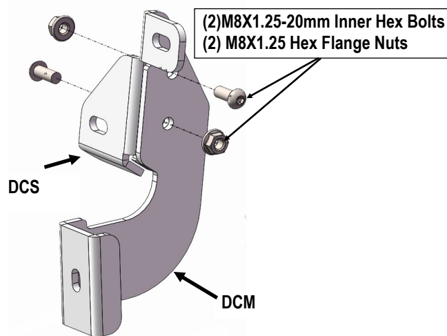
(Fig 5) Driver Center Brackets Assembly
