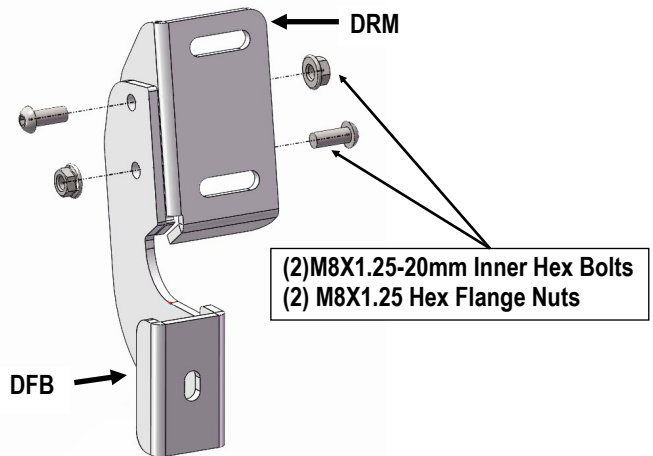
(Fig 6) Driver Rear Brackets Assembly
