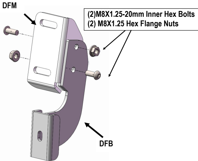
(Fig 4) Driver Front Brackets Assembly
