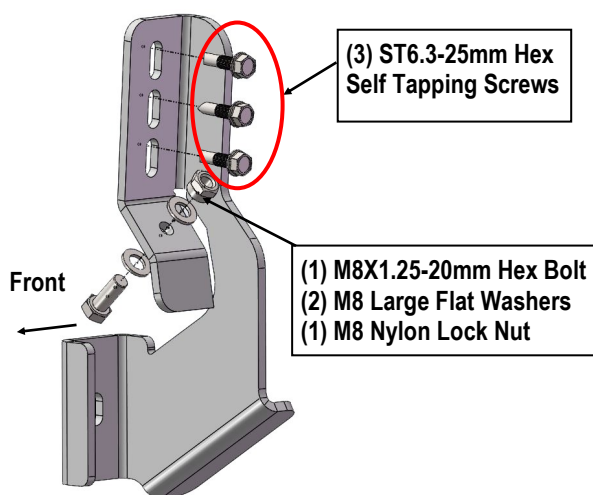
(Fig 1) Driver Side Mounting Bracket Installation Exemplified
